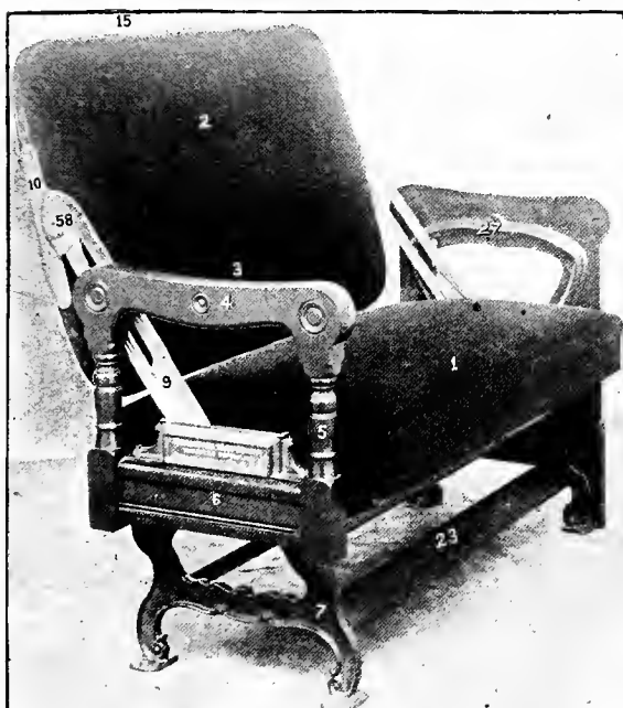
Fig. 3919. Perspective View. No. 73. HIGH-BACK TILTING CAR SEAT.
